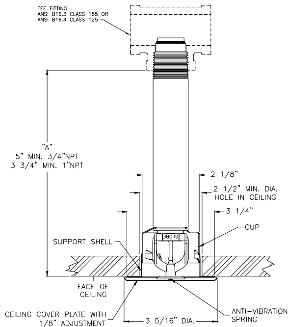
CONCEALED PENDENT
