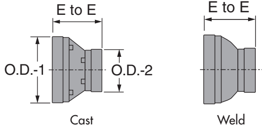
FIGURE 7072 CONCENTRIC REDUCER (GROOVE BY GROOVE)
